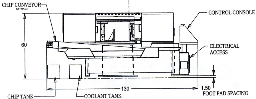
FRONT ELEVATION
